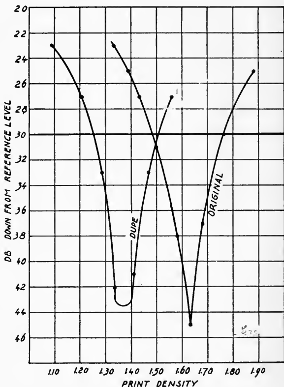
FIG. 5. Two typical cross-modulation print curves showing optima, and 30-db cancellation density range.
